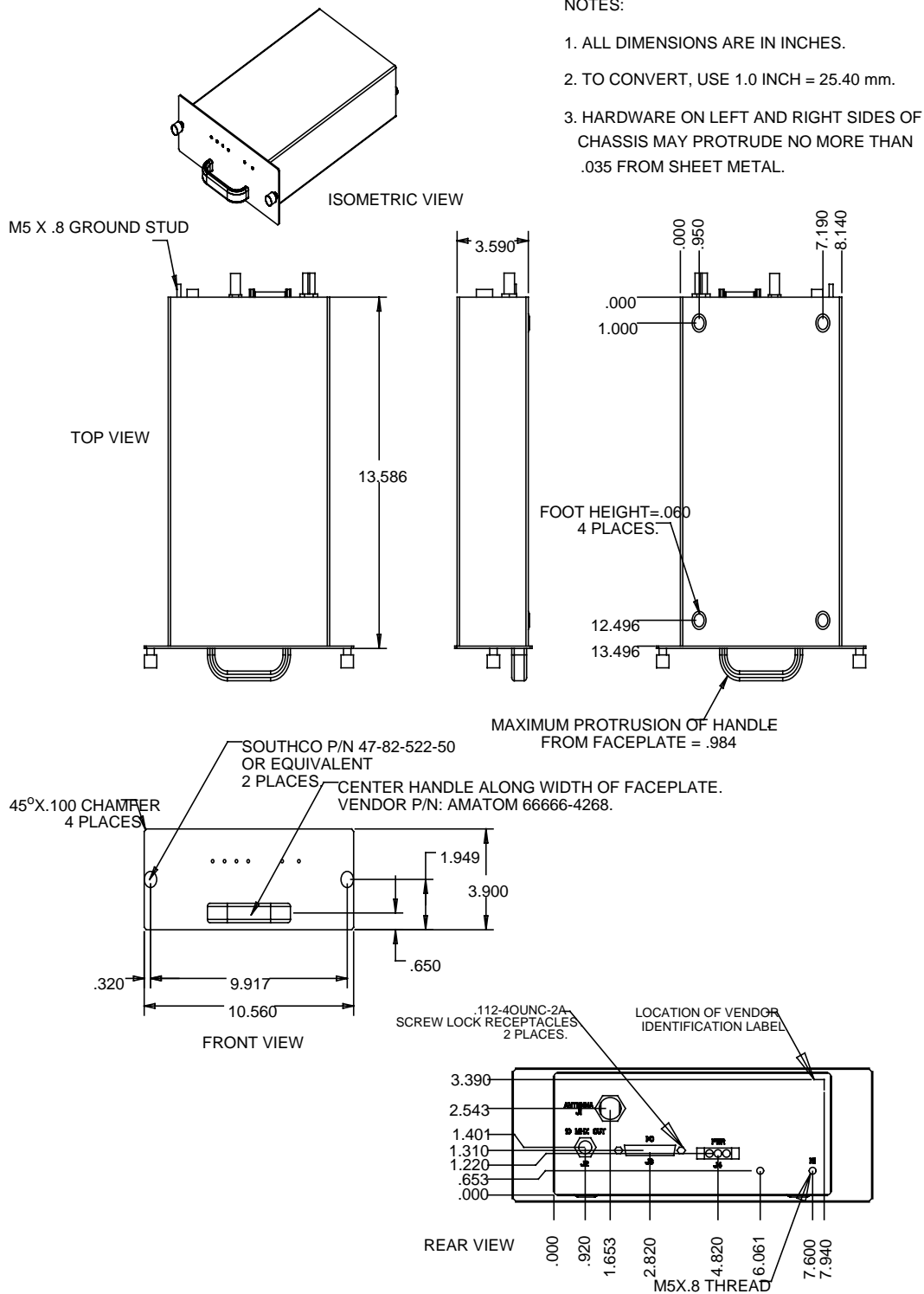
Figure 2: GPSR Outer Dimensions
